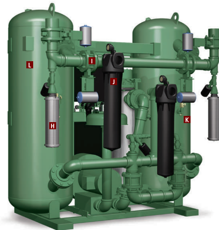
Heated Blower desiccant dryer rear view
